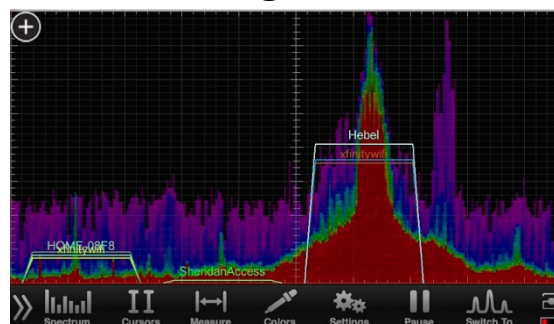
Video Streaming + Microwave Oven
